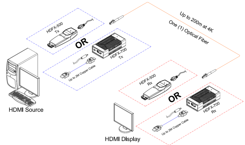
Fig Figure 3 – Connection with optical fiber
