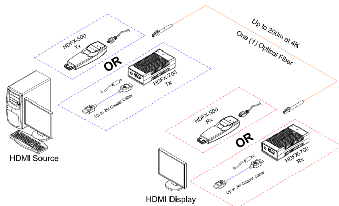
Figure 1 – Overall Connection of HDFX-500-TR
