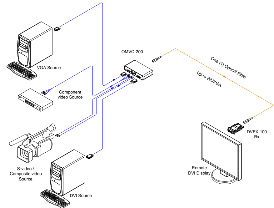
Figure 1 – Connection Diagram of OMVC-200
